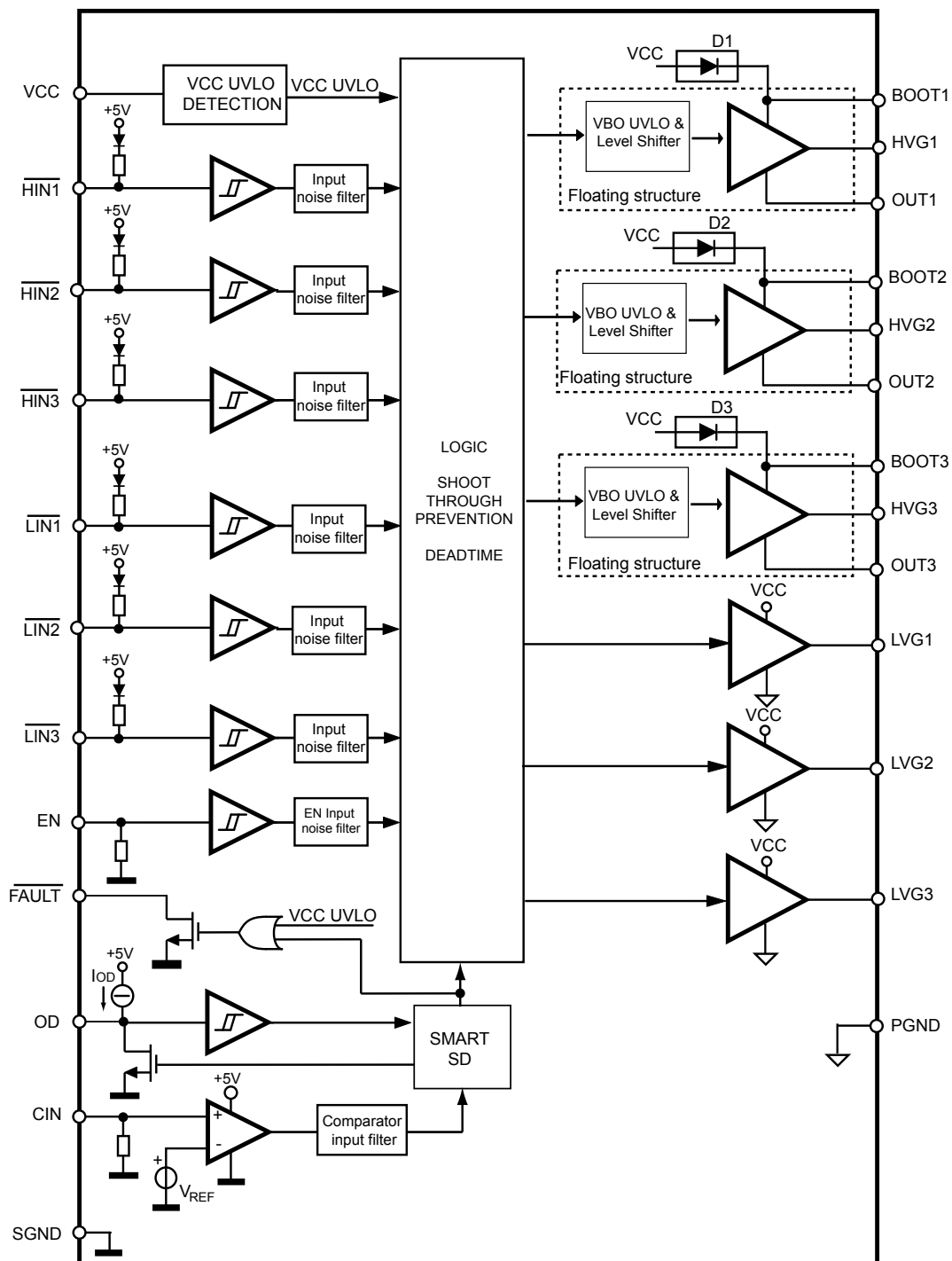
Figure 1. Block diagram
