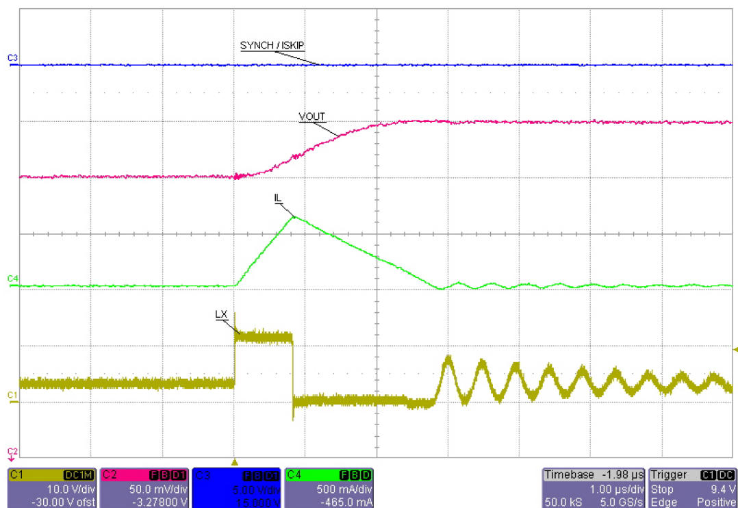
Figure 21. LCM operation with ISkip_L = 200\text{ mA} typ. at zero load
