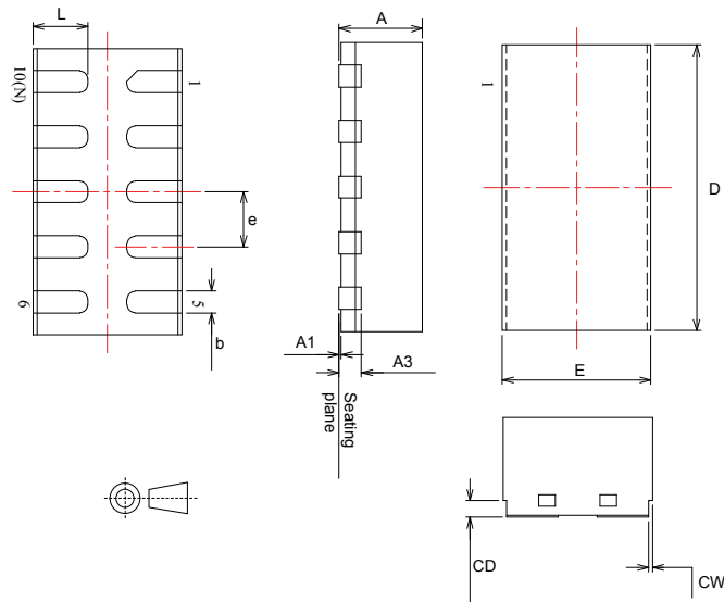
Figure 15. QFN-10L package outline
