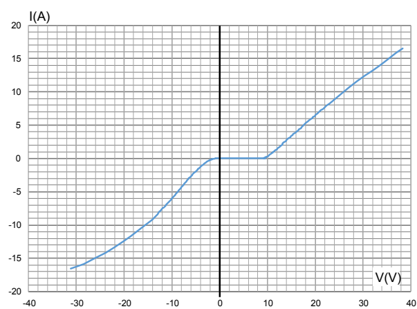
Figure 6. TLP characteristic
