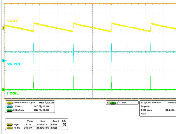
Figure 12. Output ripple, V_{IN} 3.6 V, V_{OUT} 1.8 V, I_{OUT} 1 mA
