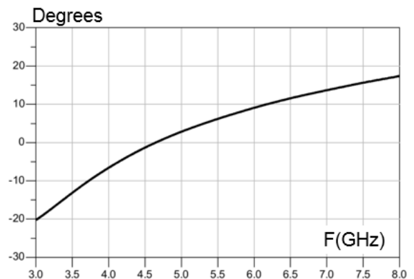
Figure 4. Phase balance (°)
