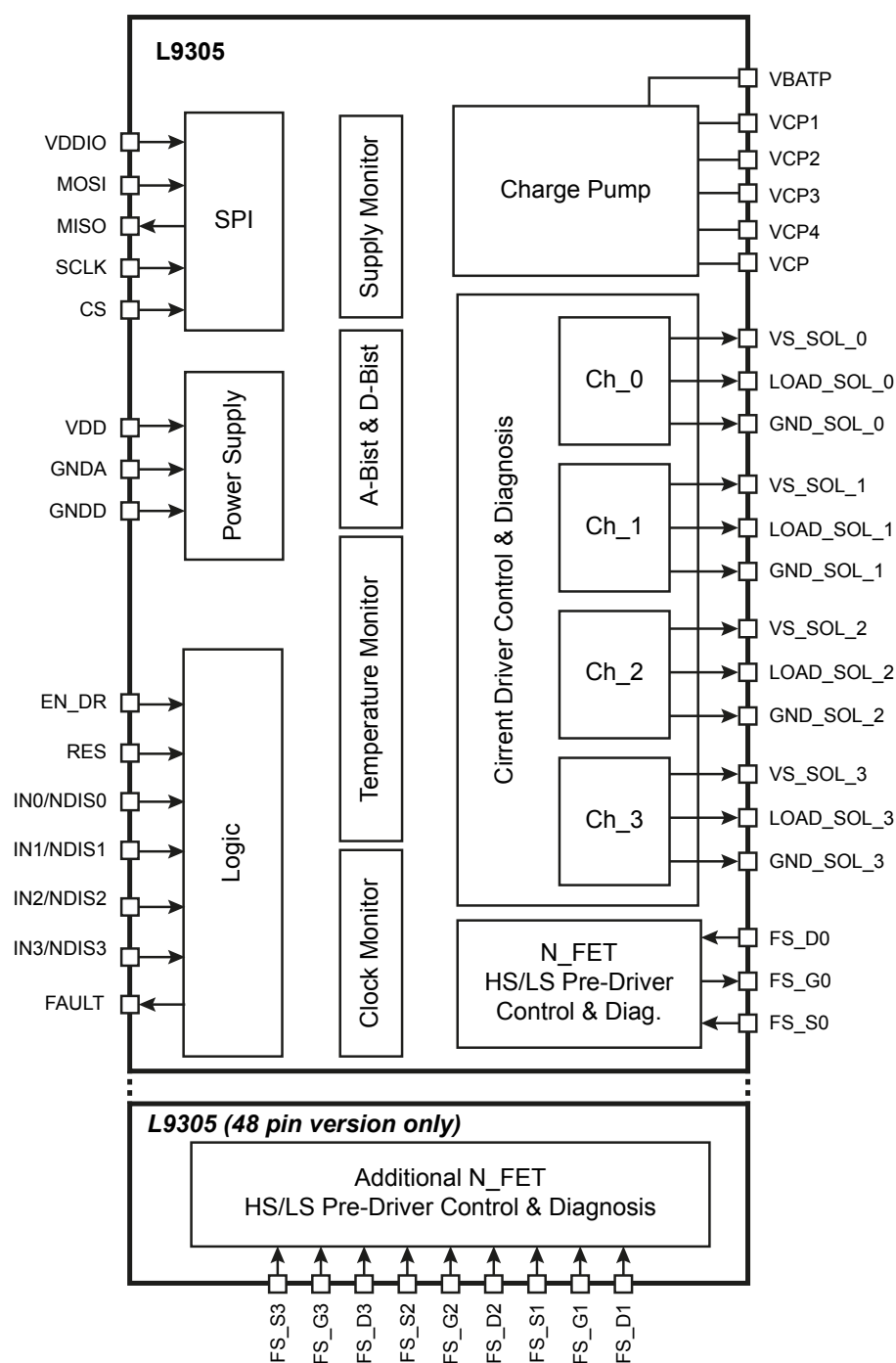
Figure 1. Block diagram
