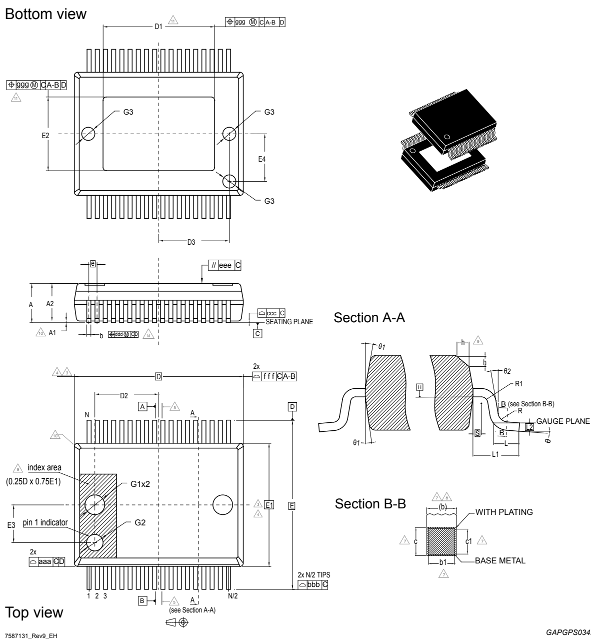
Figure 31. PowerSSO-36 (7.2x4.75 mm option C exposed pad down) package outline
