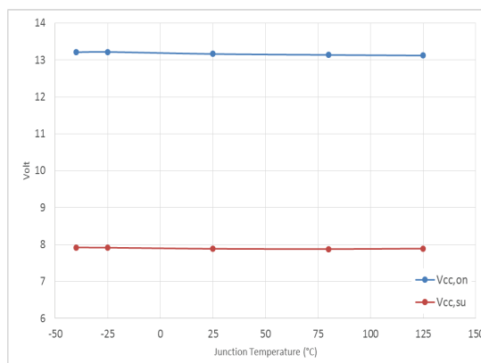
Figure 6. VCC,on and VCC,su vs. Tj
