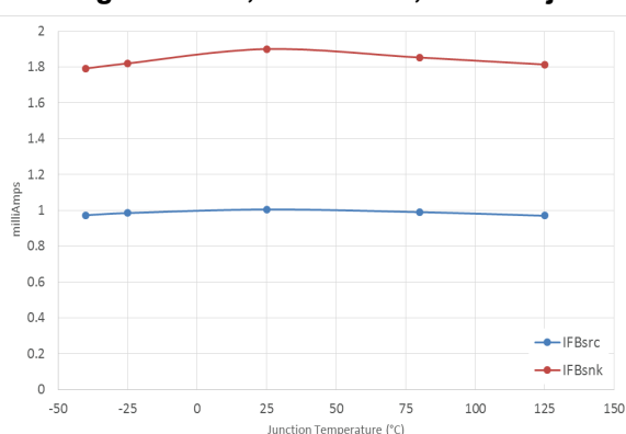
Figure 8. IFB,src and IFB,snk vs. Tj
