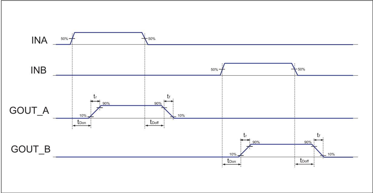
Figure 8. Timings definition
