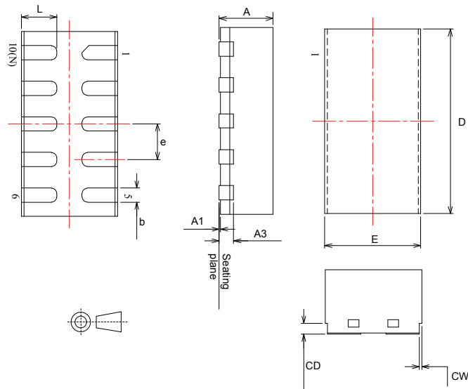
Figure 13. QFN-10L package outline
