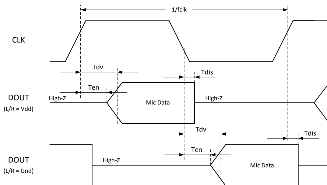
Figure 2. Timing waveforms
