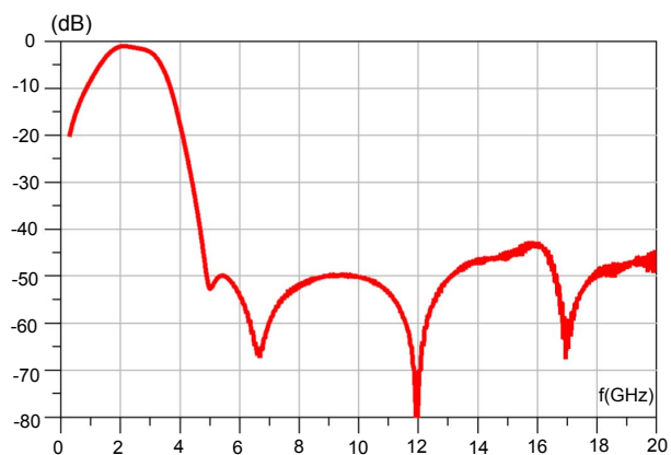
Figure 4. Transmission ( T_{\text{amb}} = 25\text{ °C} )
