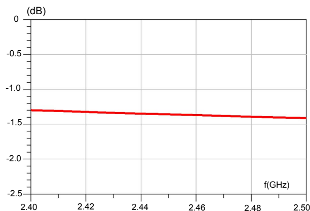
Figure 5. Insertion loss ( T_{\text{amb}} = 25\text{ °C} )
