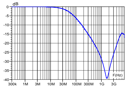
Figure 7. S21 attenuation
