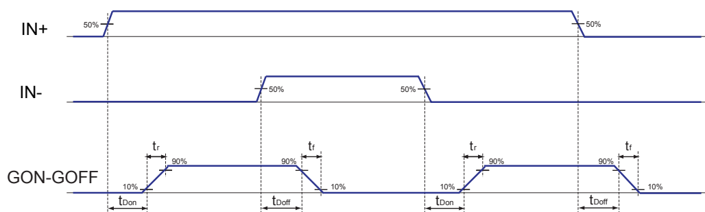
Figure 12. Timings definition
