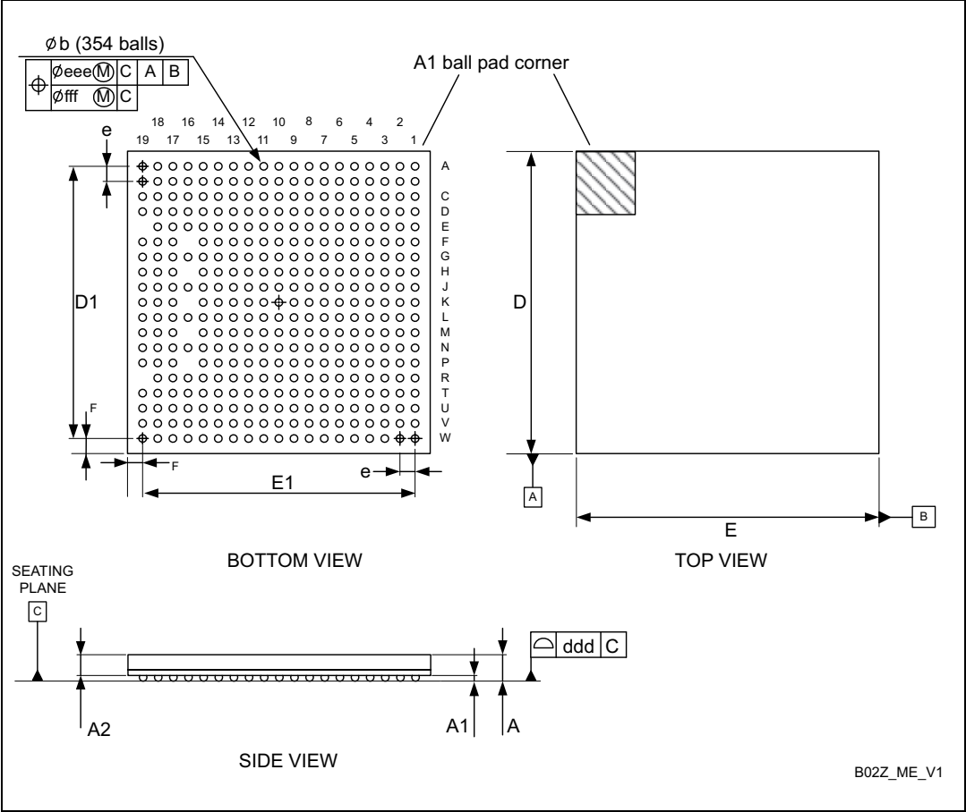
Figure 69. LFBGA354 - Outline
