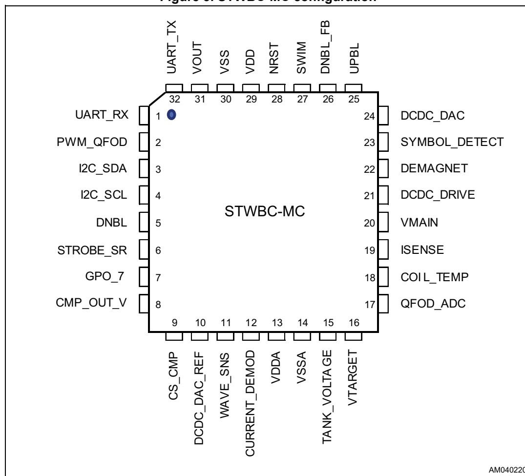
Figure 3. STWBC-MC configuration
