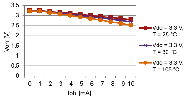
Figure 12. V_{OH} fast pad at 3.3 V
