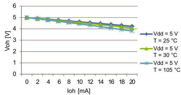
Figure 14. V_{OH} fast pad at 5 V
