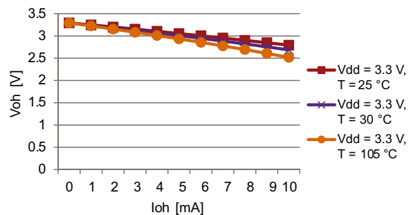
Figure 8. V_{OH} standard pad at 3.3 V
