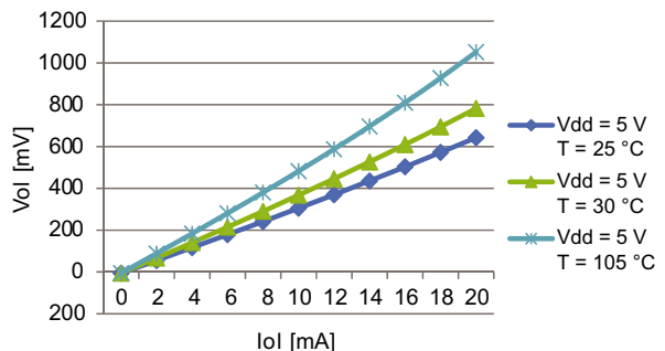
Figure 11. V_{OL} standard pad at 5 V
