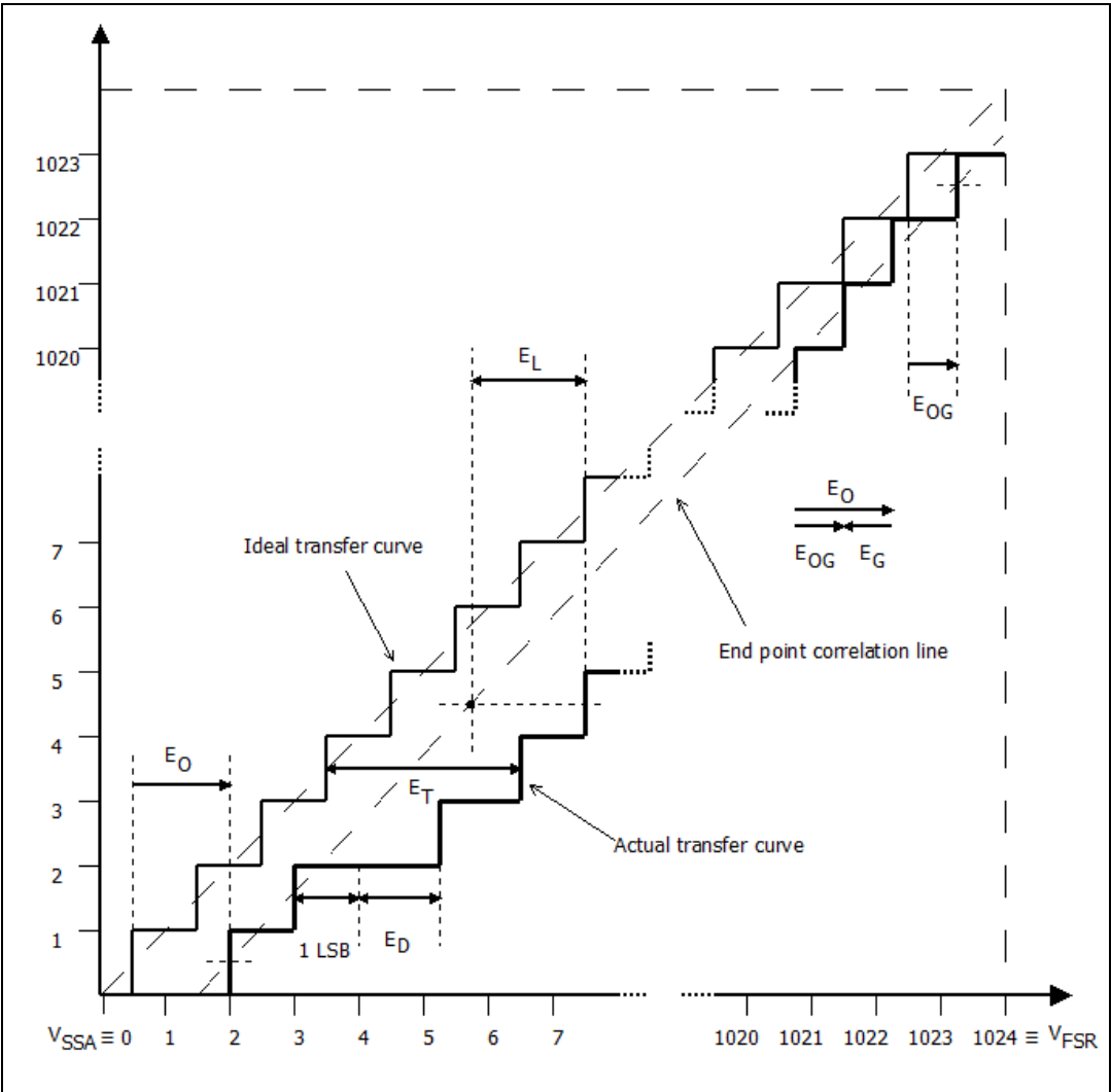
Figure 17. ADC accuracy parameter definitions
