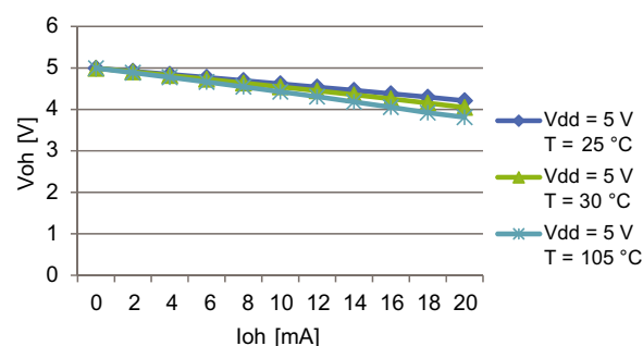
Figure 10. V_{OH} standard pad at 5 V
