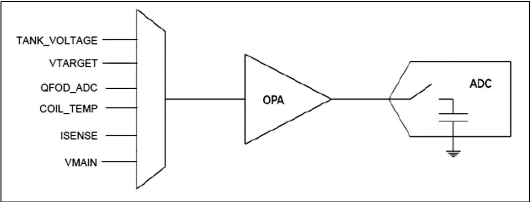
Figure 16. ADC equivalent input circuit
