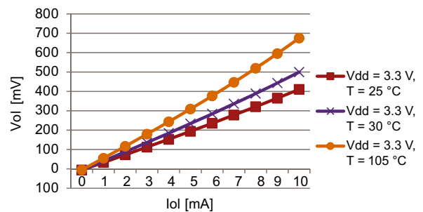
Figure 9. V_{OL} standard pad at 3.3 V
