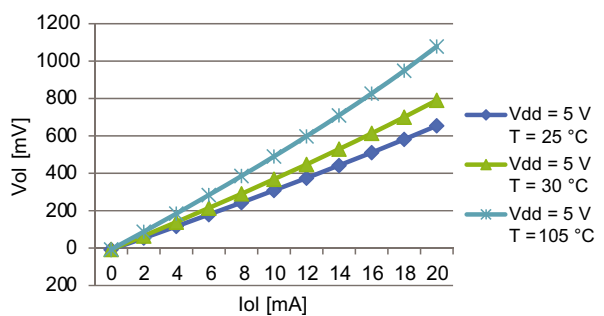
Figure 15. V_{OL} fast pad at 5 V
