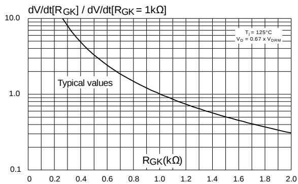
Figure 7: Relative variation of static dV/dt immunity versus gate-cathode resistance (typical values)
