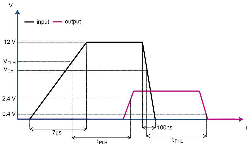
Figure 10. t_{PLH} and t_{PHL} test condition
