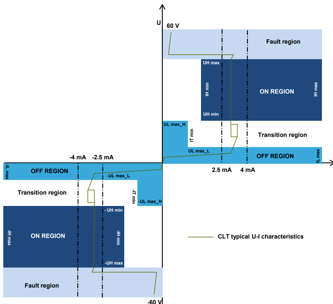
Figure 4. Input U-I operation and IEC61131-2 characteristic limits
