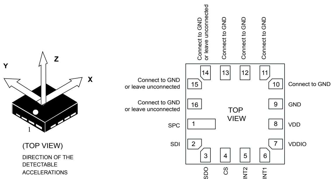
Figure 1. Pin connections
