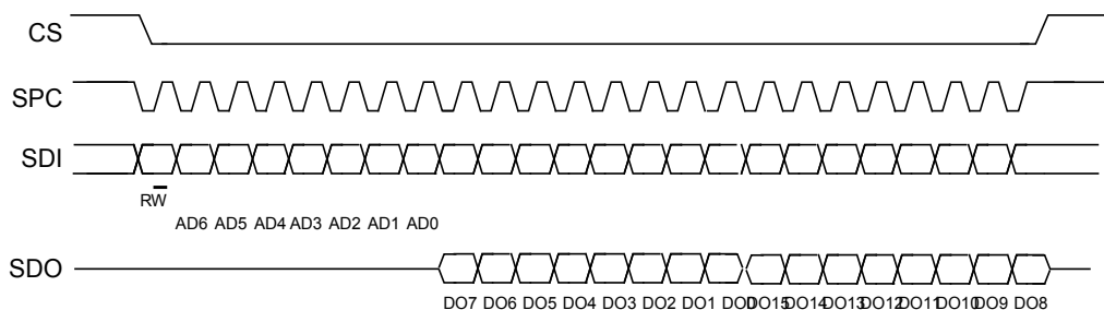
Figure 6. Multiple byte SPI read protocol (2-byte example)
