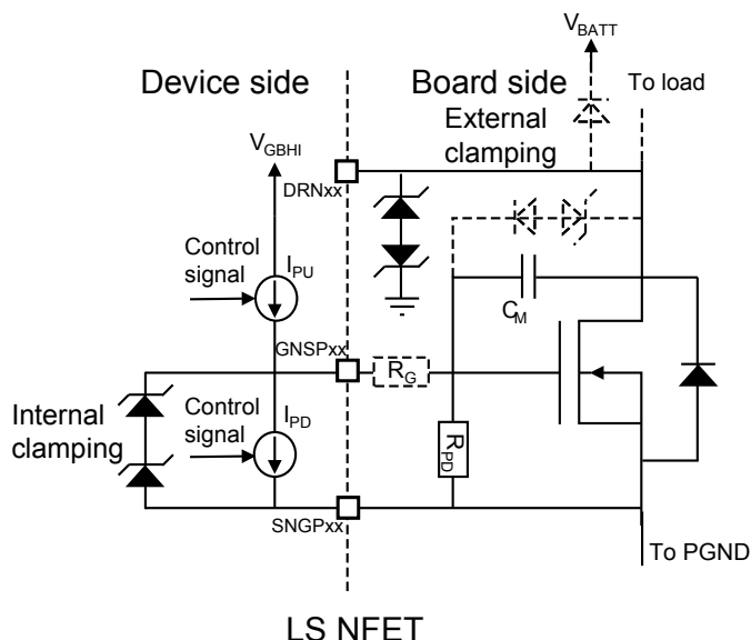
Figure 14. Clamping for LS configuration
