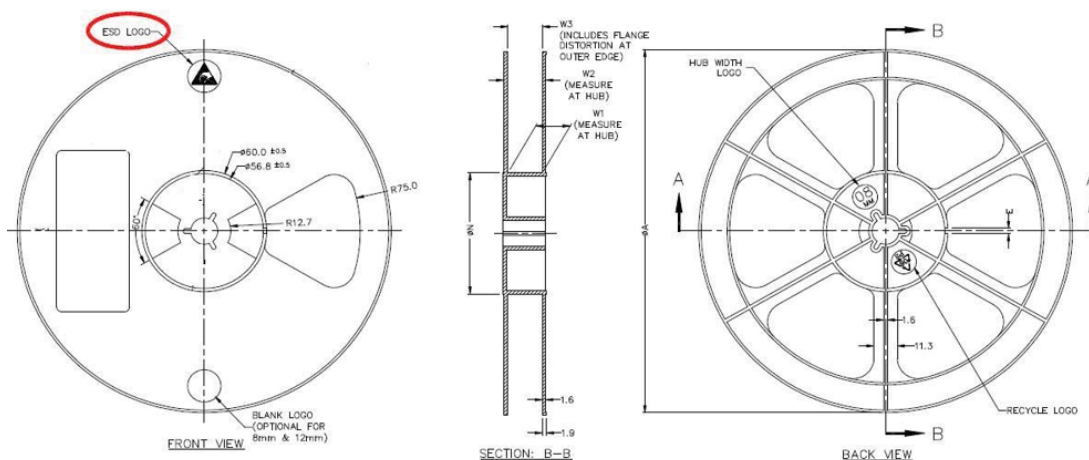
Figure 25. DFN4 1x1 reel outline
