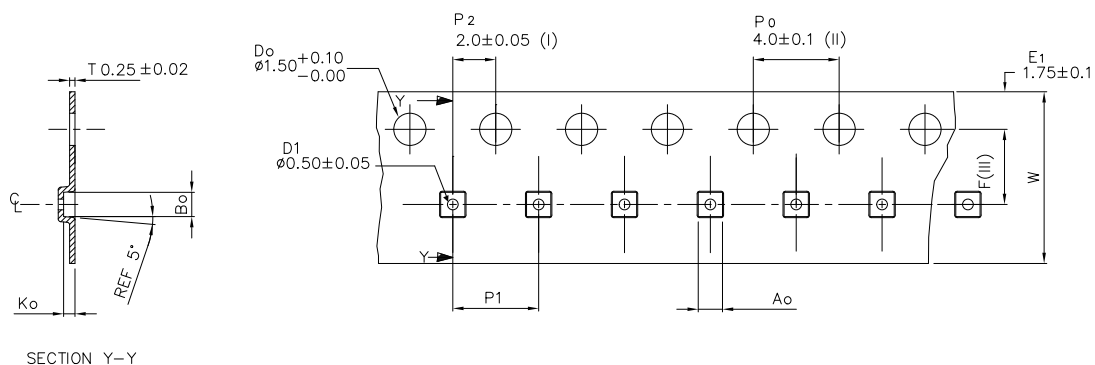
Figure 24. DFN4 1x1 tape outline
