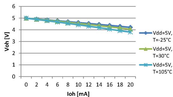
Figure 11. V_{OH} standard pad at 5 V
