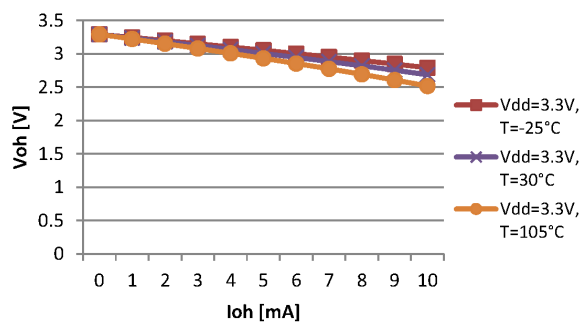
Figure 9. V_{OH} standard pad at 3.3 V
