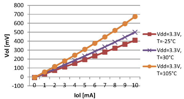
Figure 10. V_{OL} standard pad at 3.3 V
