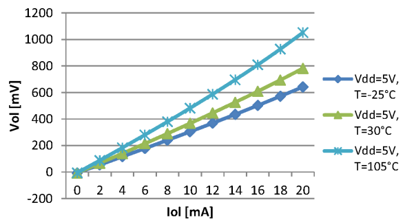
Figure 12. V_{OL} standard pad at 5 V
