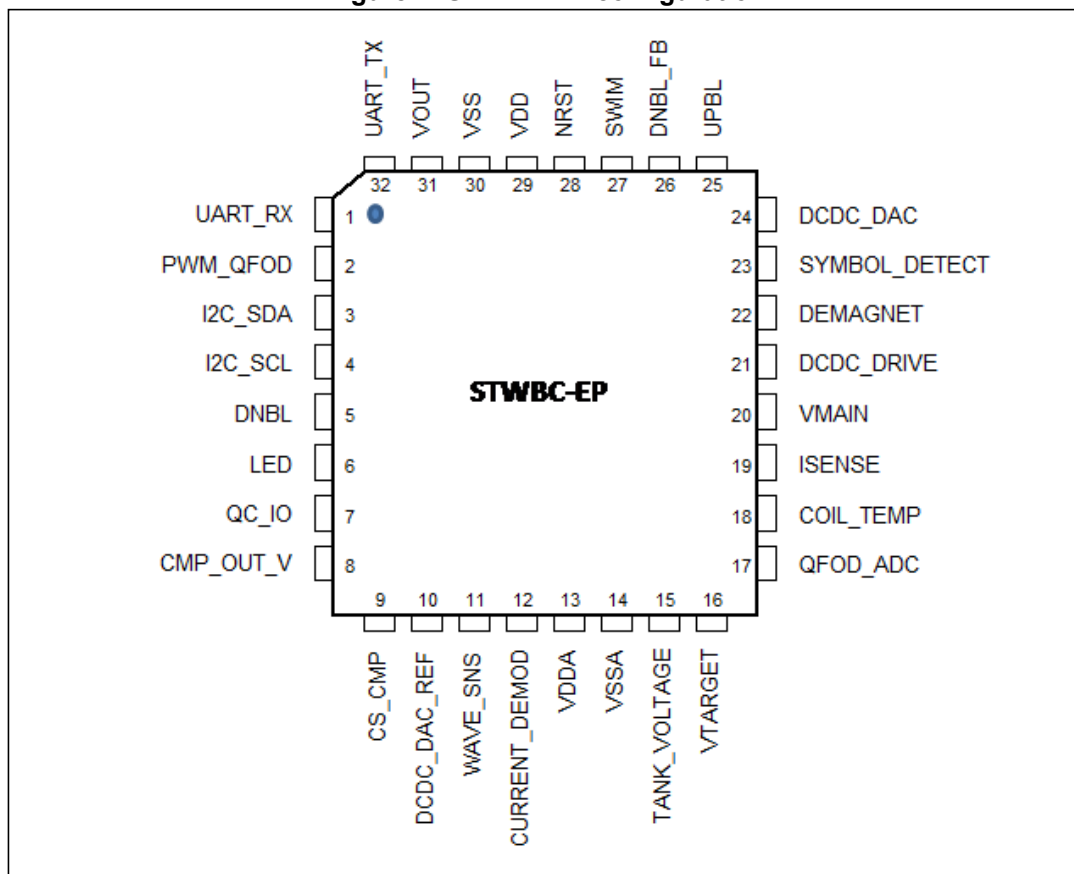
Figure 4. STWBC-EP configuration
