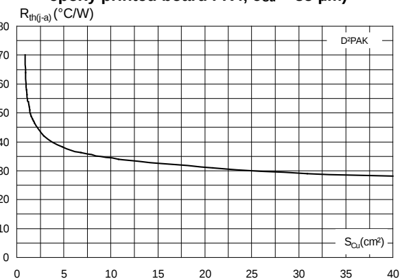
Figure 8: Thermal resistance junction to ambient versus copper surface under tab (typical values, epoxy printed board FR4, e_{Cu} = 35 \mu m )
