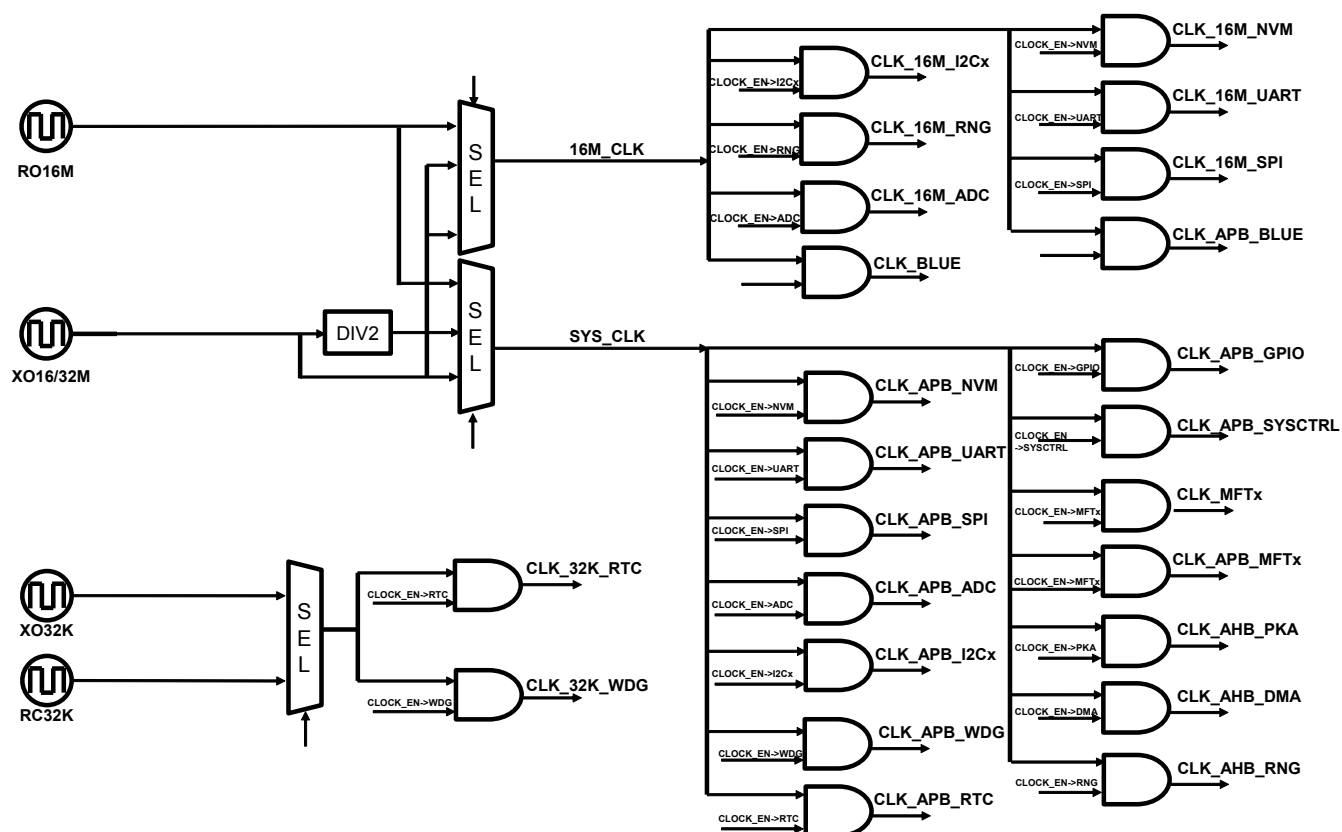
Figure 6. Clock tree
