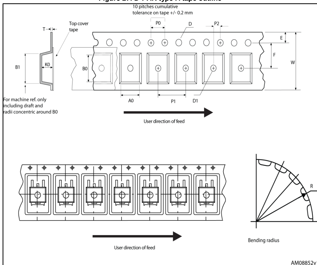
Figure 27: D 2 PAK type A tape outline
