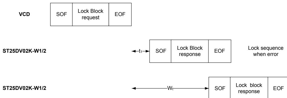
Figure 16. Lock single block frame exchange between VCD and ST25DV02K-W1/2
