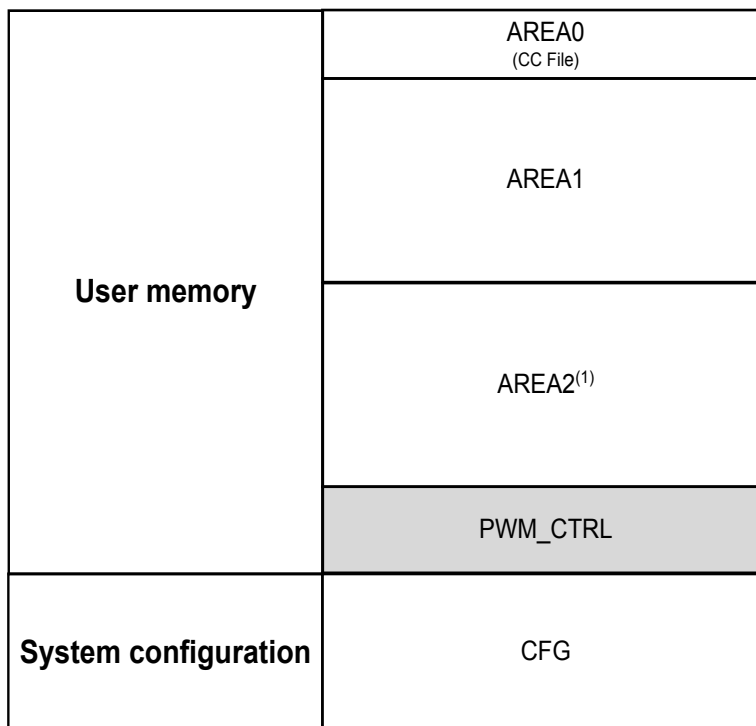
Figure 5. Memory organization
