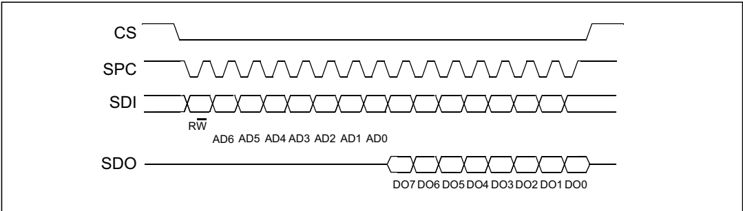
Figure 15. SPI read protocol
