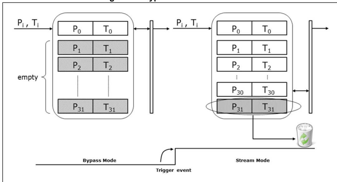
Figure 11. Bypass-to-Stream mode
