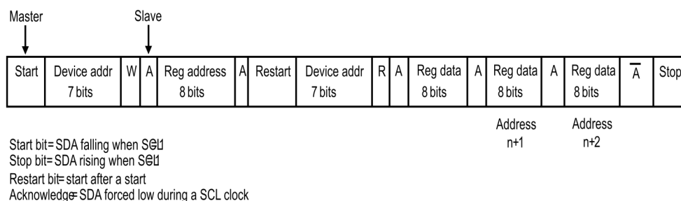
Figure 4. Read operation
