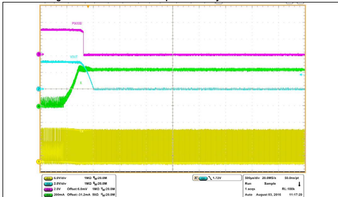
Figure 25. Valley current sense implements constant current protection
