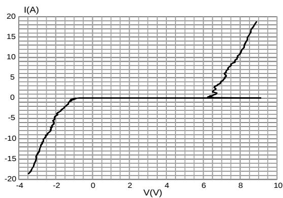
Figure 7: TLP characteristic
