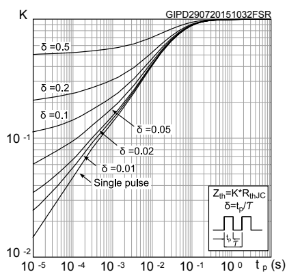
Figure 15. Thermal impedance
