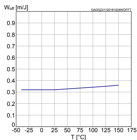
Figure 29. Woff vs. Tcase
