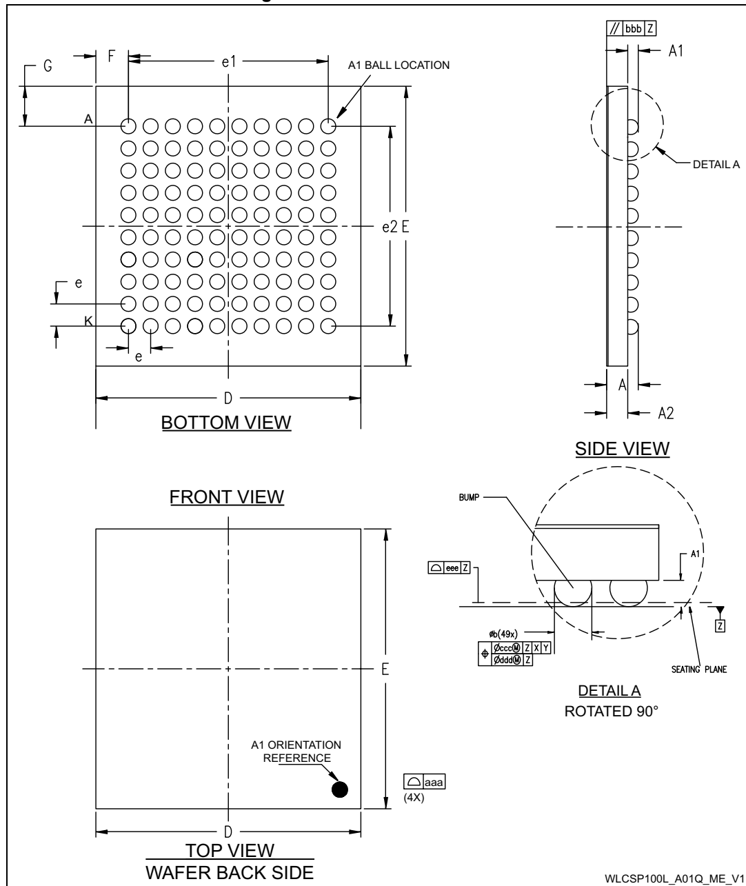
Figure 96. WLCSP100 outline
