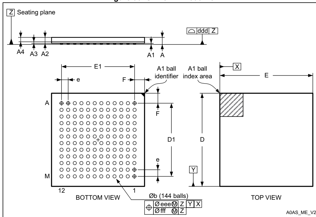
Figure 90. UFBGA144 outline
