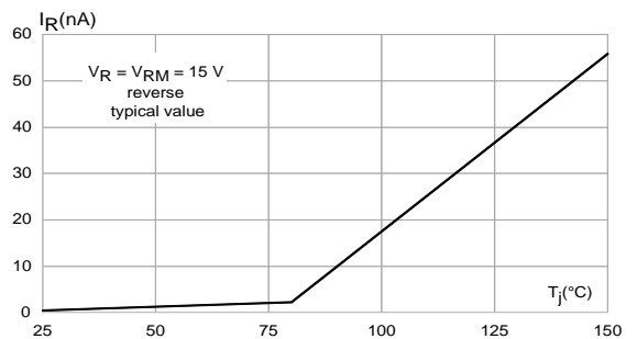
Figure 6: Leakage current versus junction temperature (typical value)
