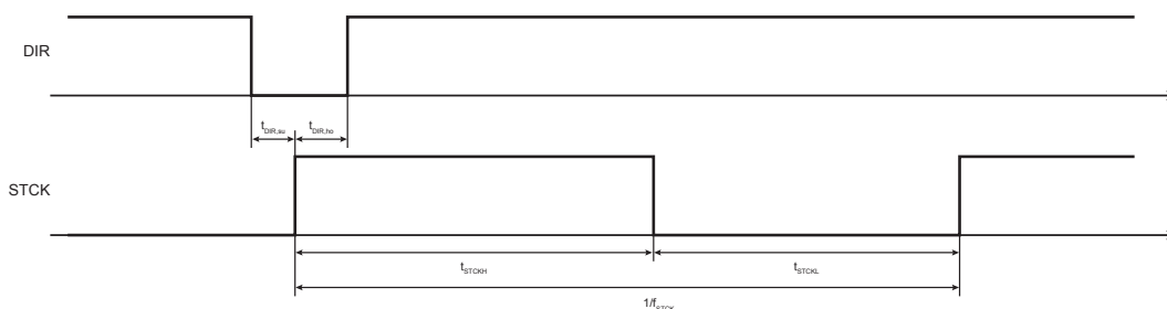
Figure 4. STCK and DIR timing
