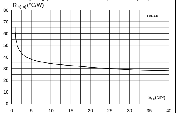
Figure 8: Thermal resistance junction to ambient versus copper surface under tab (typical values, epoxy printed board FR4, e_{Cu} = 35 \mu m )
