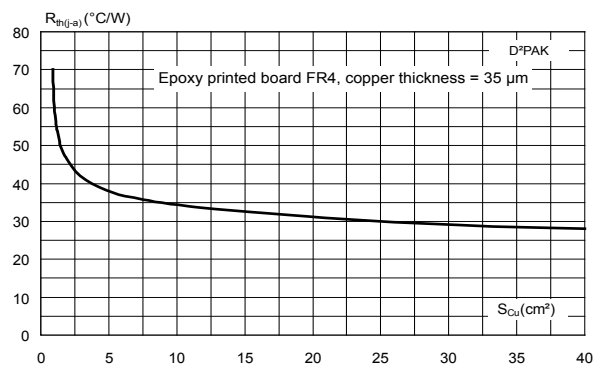
Figure 11. Thermal resistance junction to ambient versus copper surface under tab for D²PAK package (typical values)
