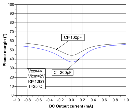
Figure 23. Phase margin vs. output current at V_{CC} = 4\text{ V}
