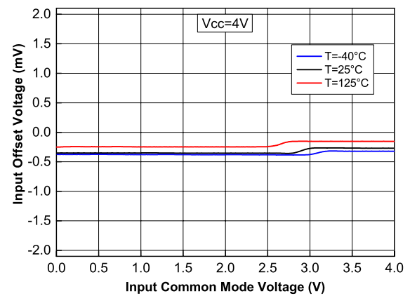
Figure 10. Input offset voltage vs. common-mode voltage at V_{CC} = 4\text{ V}
