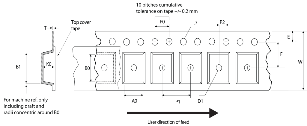
Figure 19. D 2 PAK tape outline
