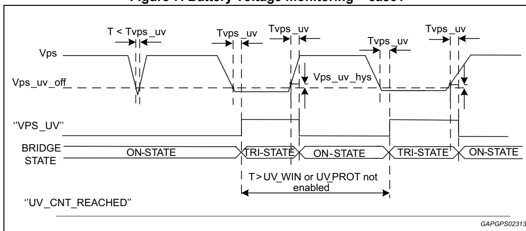
Figure 7. Battery voltage monitoring – case1
