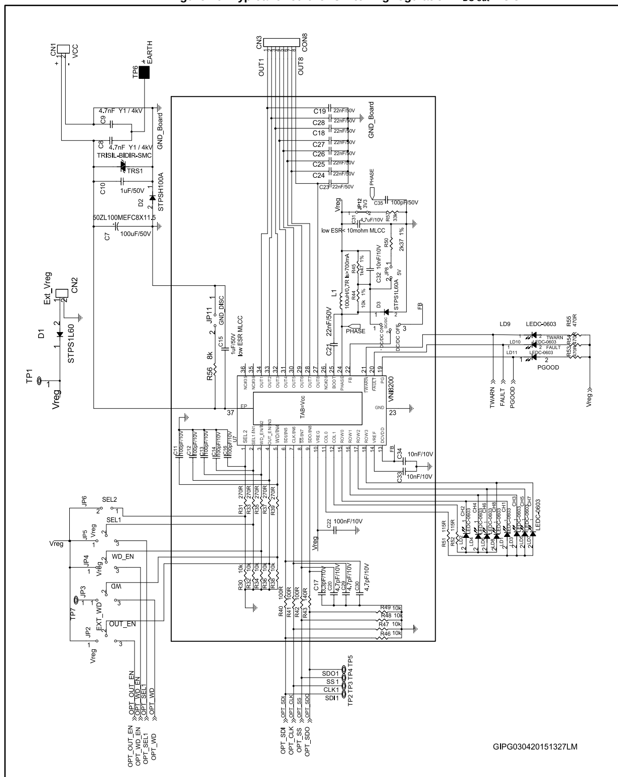
Figure 10: Typical circuit for switching regulation V_{DC-out} = 3.3\text{ V}
