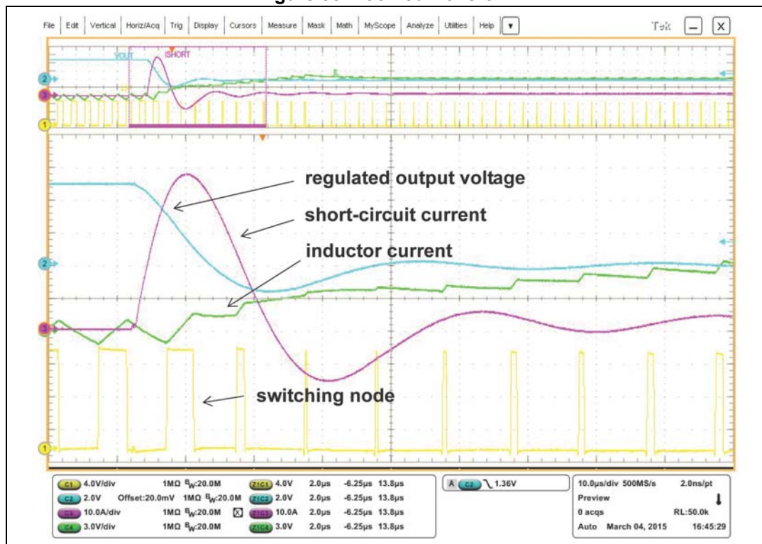
Figure 33. Zoomed waveform
