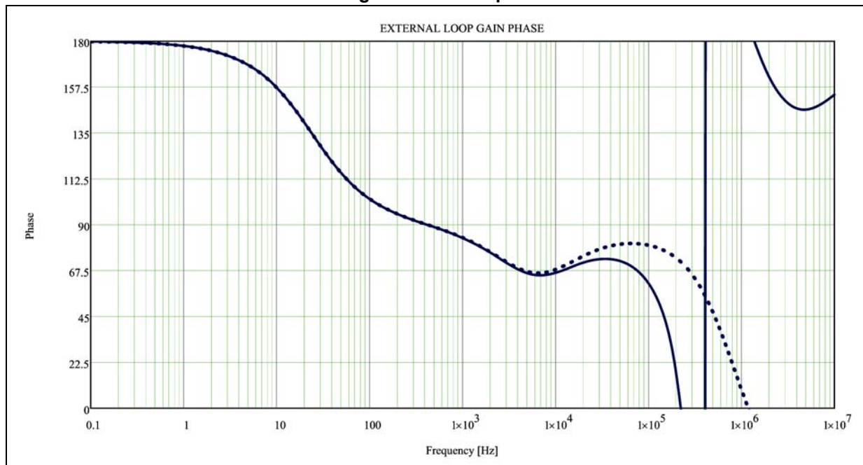
Figure 40. Phase plot
