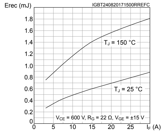
Figure 12. Diode reverse recovery energy vs forward current
