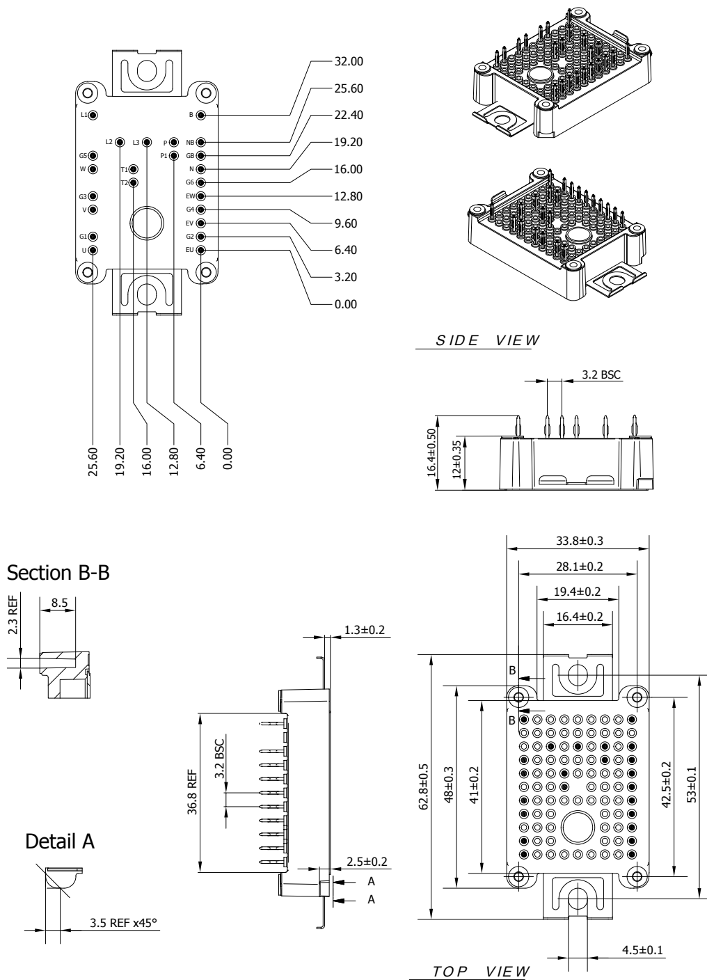
Figure 23. ACEPACK™ 1 CIB press fit pins package outline (dimensions are in mm)
