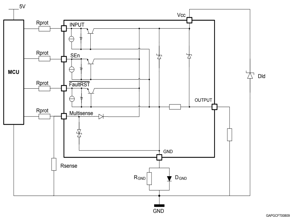
Figure 36. Simplified internal structure
