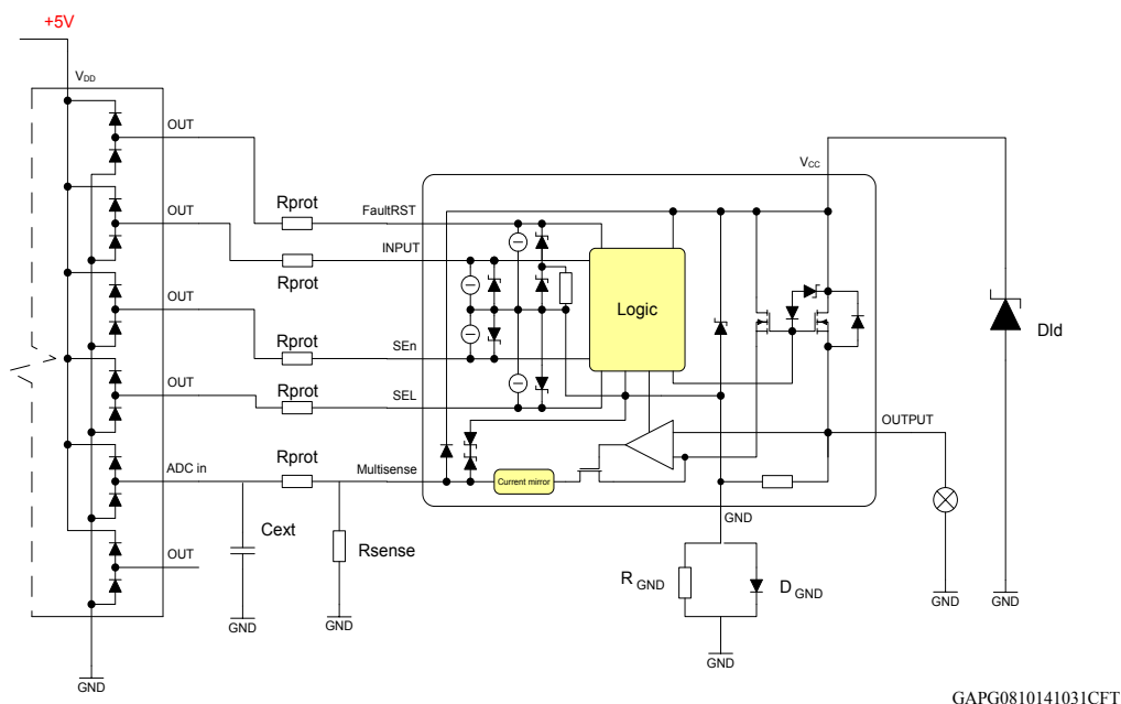
Figure 35. Application diagram
