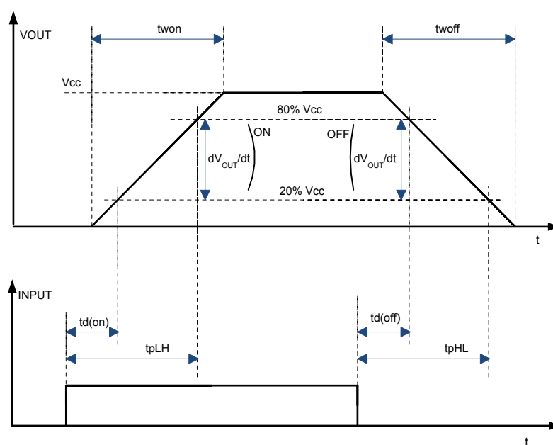
Figure 6. Switching time and pulse skew
