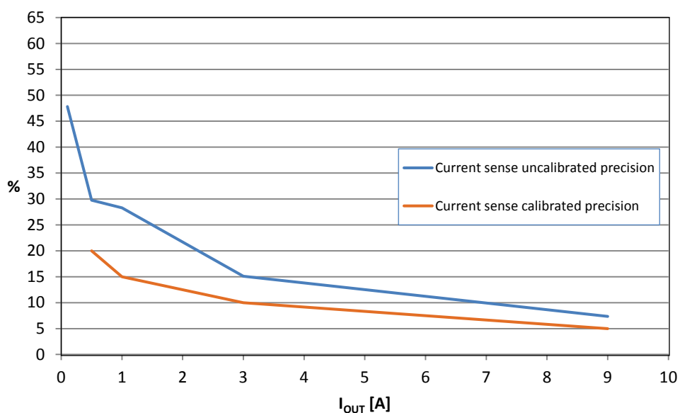
Figure 5. Current sense accuracy versus I_{OUT}
