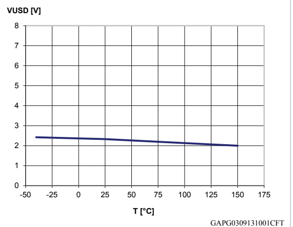
Figure 24. Undervoltage shutdown
