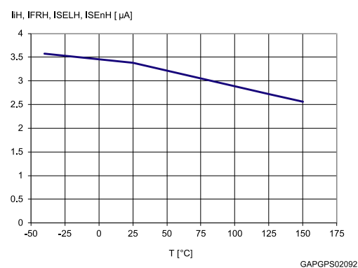
Figure 20: High level logic input current
