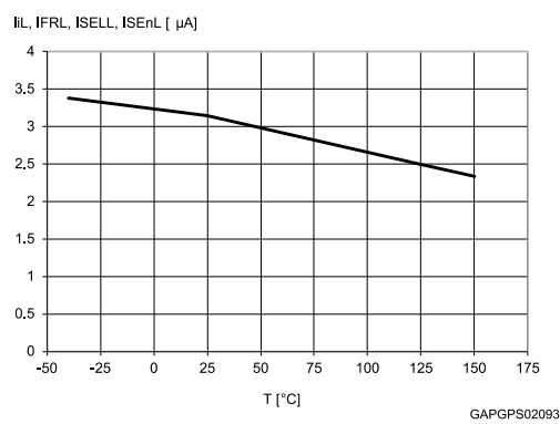
Figure 21: Low level logic input current
