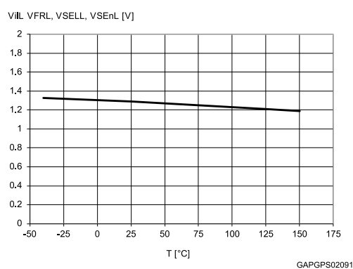
Figure 19: Logic Input low level voltage
