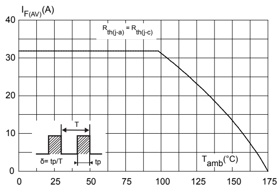
Figure 2. Average forward current versus ambient temperature (δ = 0.5, anode terminals short circuited)
