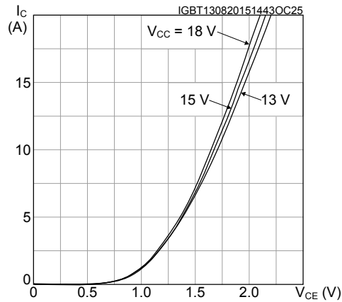
Figure 11. Output characteristics
