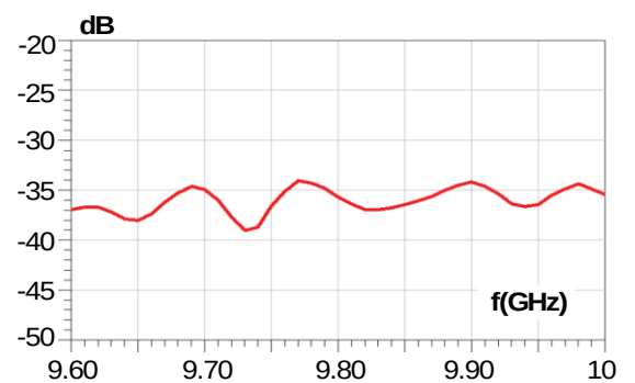
Figure 8: H4 filtering
