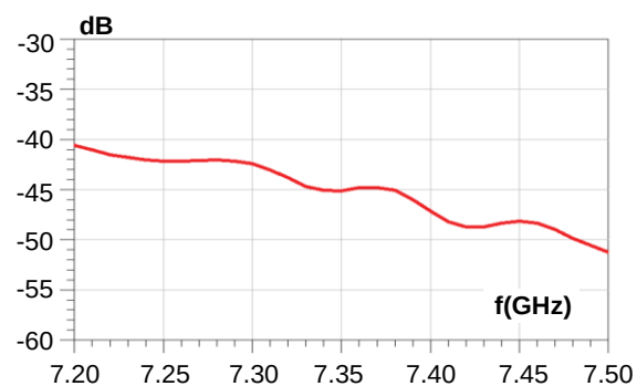
Figure 7: H3 filtering
