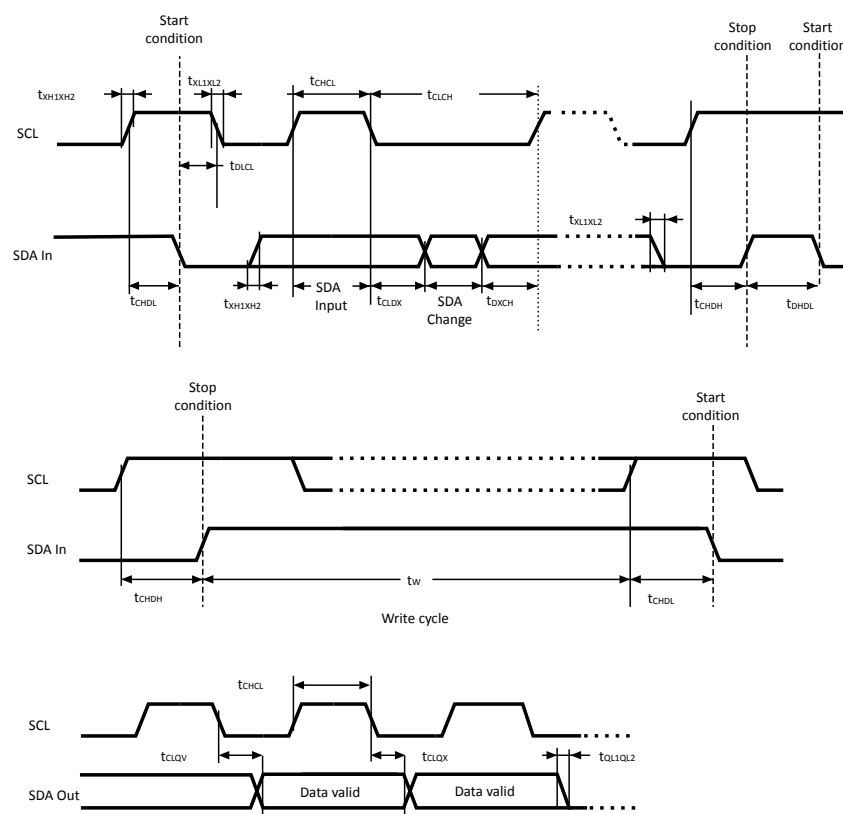
Figure 11. AC waveforms
