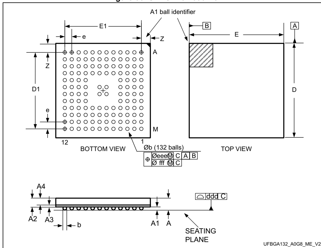
Figure 36. UFBGA132 outline
