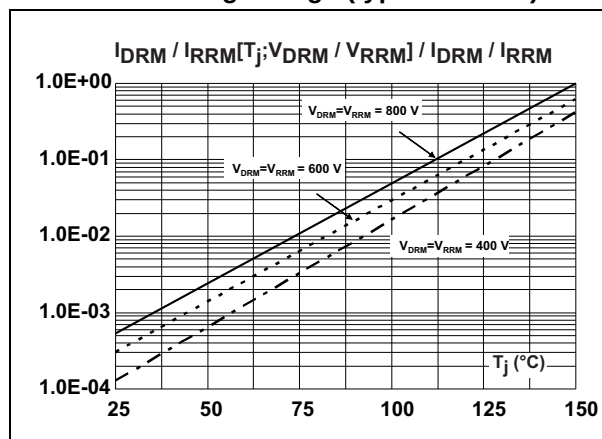
Figure 14. Relative variation of leakage current versus junction temperature for different values of blocking voltage (typical values)
